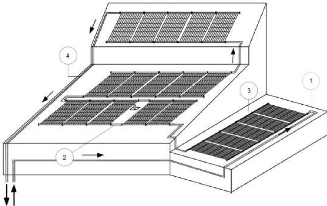
Figure 3.1: Sample collector system
